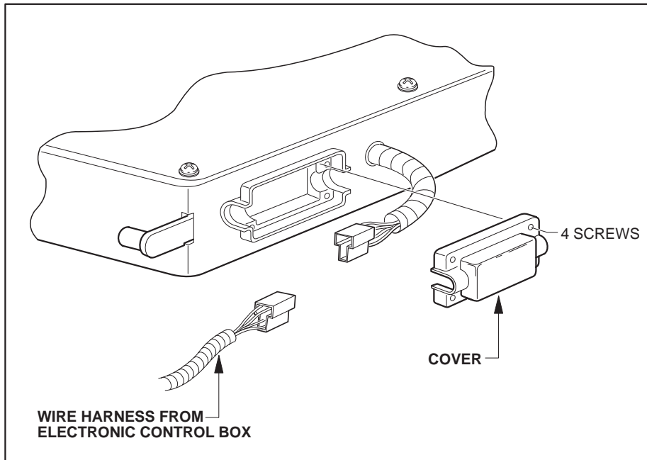
VIEW A
