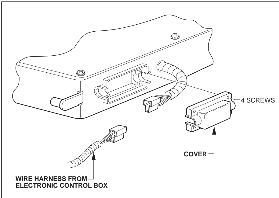
VIEW A
